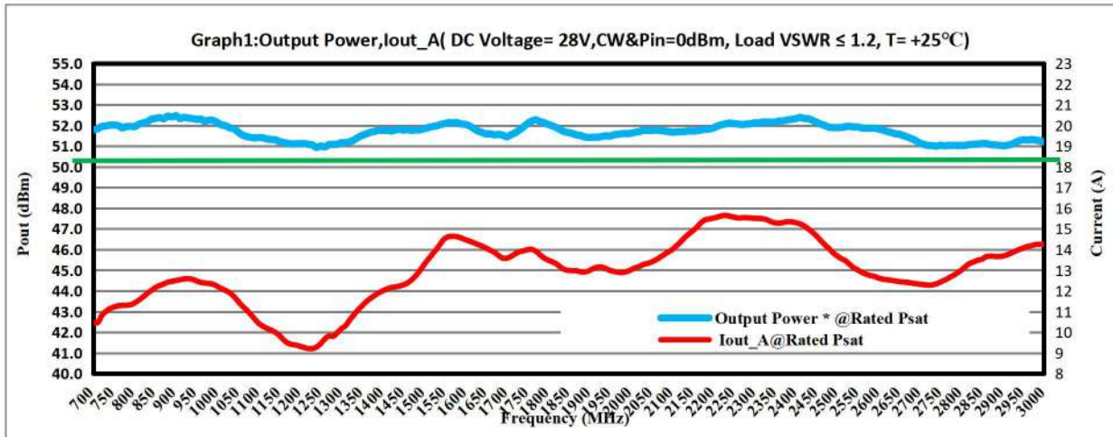
Pout & Power Consumption [Pin=0 dBm, CW, Load VSWR≤1.2, 25°C]
