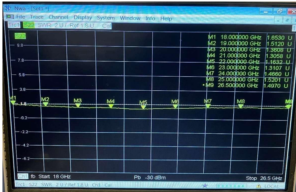
Output VSWR @ Pin=-30 dBm (Ambient temp. +25±3°C, DC Voltage= 24V)
