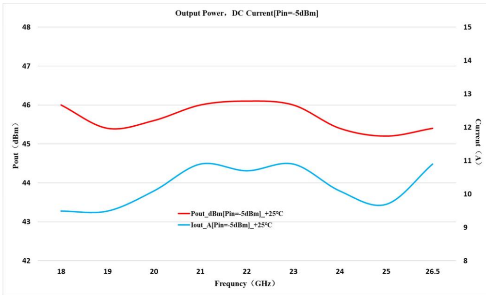
Output Power (CW, Normal temp. +25±3°C)
